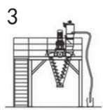
配置3: 真空上料, 负压吸料; Config 3: Use a vacuum feeder to feed.
