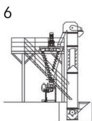
配置6: 斗式提升机加料, 省空间; Config 6: Bucket elevator feeding.
