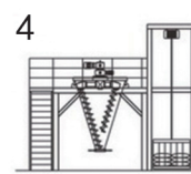
配置4: 架设货梯平台, 人工入料; Config 4: Manual feeding, freight elevator platform lifting.
