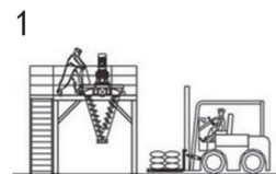
配置1: 简易操作平台, 装运叉车配合操作; Config 1: Use a forklift to cooperate with the operation.
