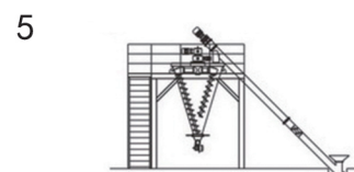
配置5: 架设螺旋输送机使用, 简易投料; Config 5: Feeding with screw conveyor.
