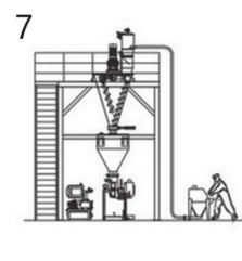
配置7: 与真空加料, 包装机等配套使用; config 7: Use with vacuum feeding, packing machine, etc.
